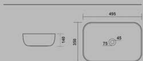
7030-COREL L 495 W 350 H 140mm
